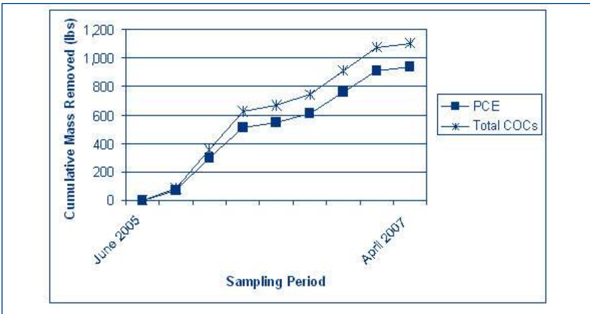
Figure 1. To date, the Riverfront OUI ART system has removed approximately 83% of the source-area VOCs.
